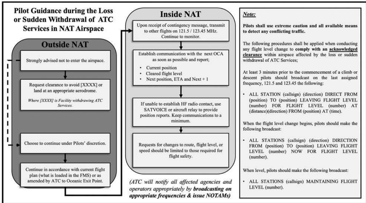
Figure 11-3 — Visual aid for pilot guidance during loss or sudden withdrawal of ATC services in NAT airspace.
