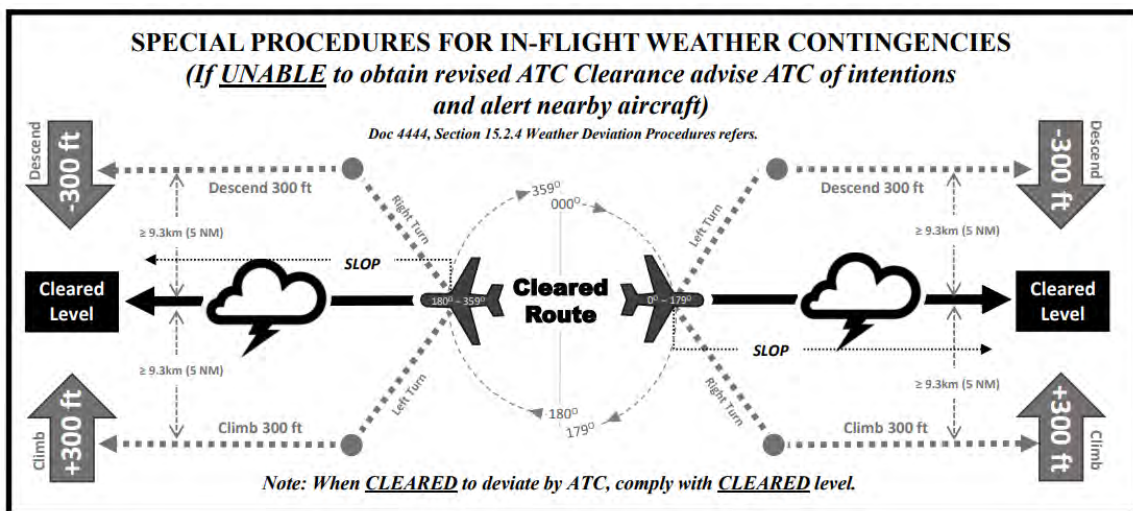
Figure 11-2. Visual aid for understanding and applying the weather contingency procedures guidance.
