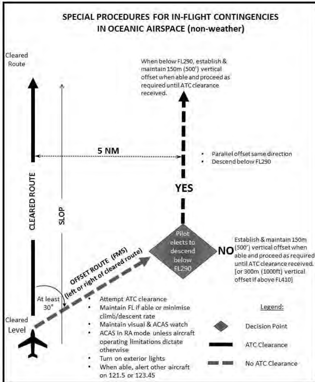
Figure 11-1 — Visual aid for understanding and applying the contingency procedures guidance.
