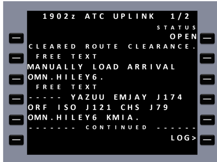
Figure 27. UM80 Clearance Uplink with Free Text Arrival – DAT Code 1FANSER2PDC or FANSER Example
