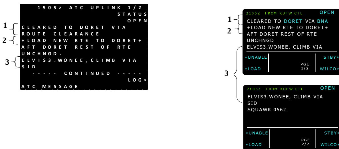
Figure 15. Depiction of Revised CPDLC DCL Including “REST OF ROUTE UNCHANGED”
