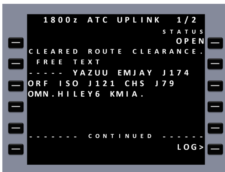
Figure 24. UM80 Full Route Clearance and Supplementary Route Free Text (B737 MCDU Test Bench – FAA Tech Center)
