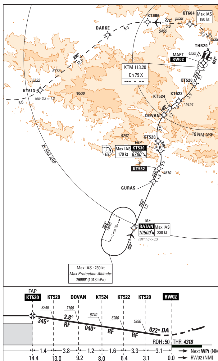
Figure 4 Example of RNP AR approach chart.
